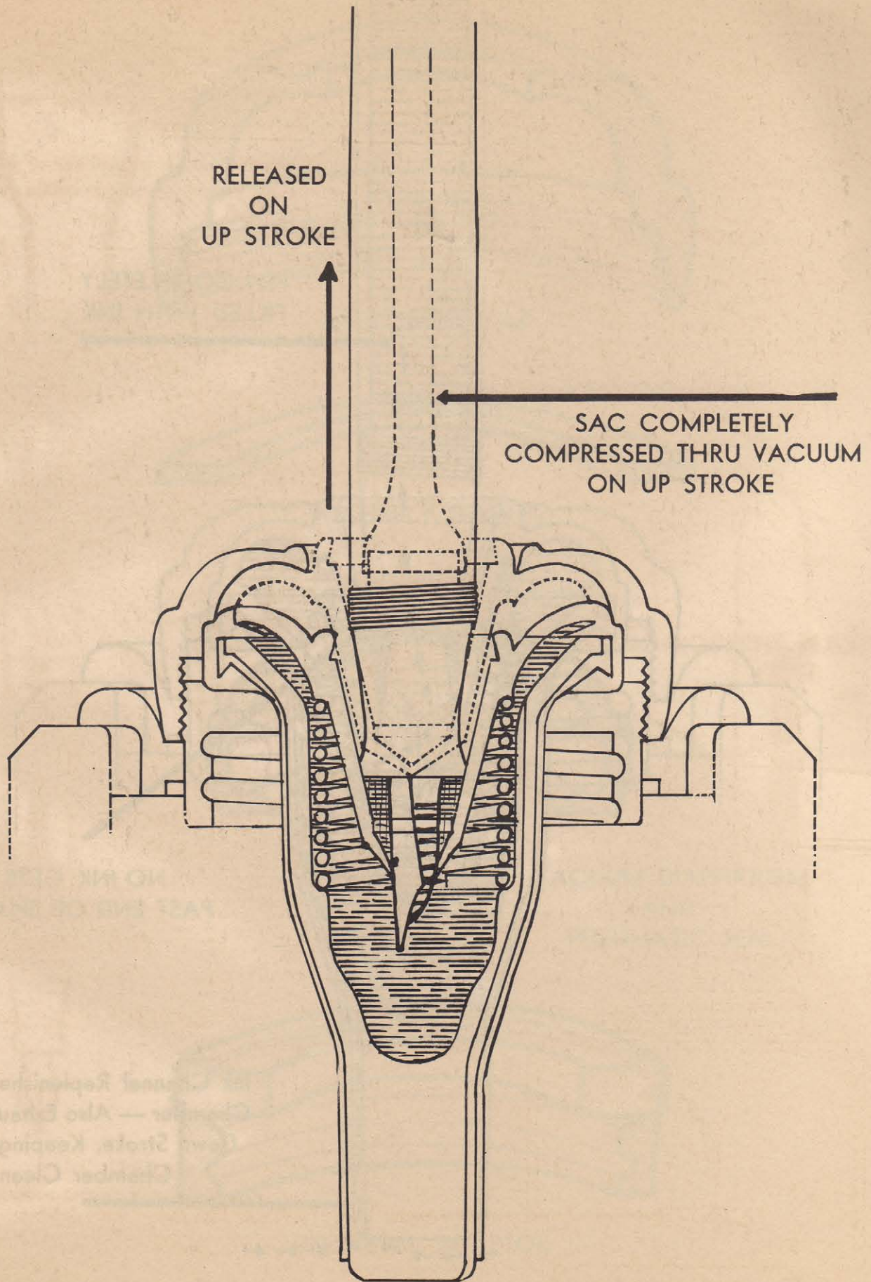
THIRD—Pen released, Penfiller evacuating air completely.
